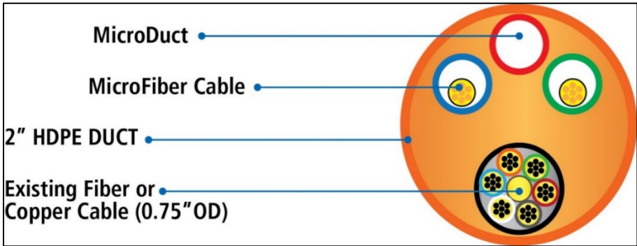
Figure 7: HDPE Outer Duct with Inner Duct and Microducts
