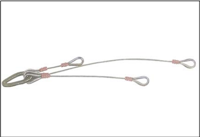
Figure 4: Staggered Pulling Harness for Pulling Multiple Cables or Innerducts
