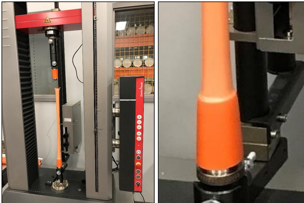
Figure 1: Example of Conduit Pulled Past Yield Point (Left: Full test Rig after Elongation/Break, Right: Closeup of Transition from Unyielded to Yielded Conduit)
