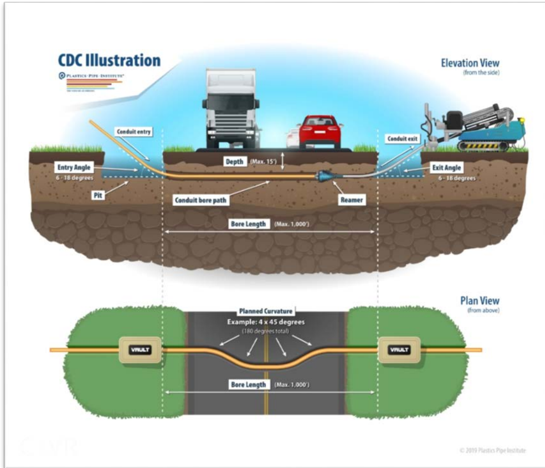
Figure 1 - Schematic of Typical Mini-HDD Installation
