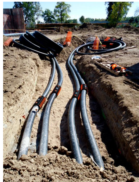
Four parallel, five-inch diameter, pre-insulated PEX pipes are laid out side-by-side for supply of heated fluid for snow melting and radiant heating within the new Asian Tropics complex. These flexible pipes follow the contours of the land over long distances.
