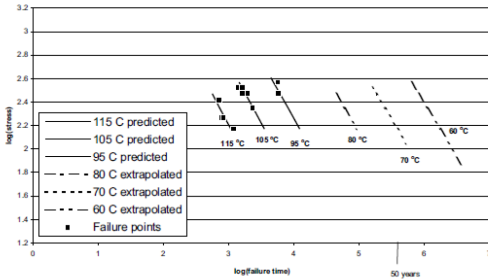
Figure 5: Failure Times for a PEX Pipe Material Exposed to Chlorinated Potable Water
